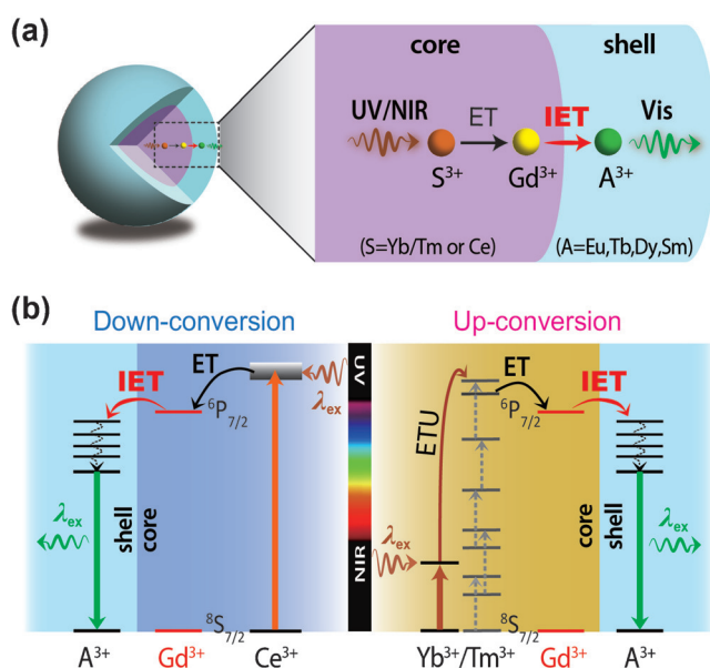
Figure 1. a) Proposed mechanism of photon up- and down-conversion through Gd^{3+} -mediated interfacial energy transfer in a core-shell architecture design. b) Schematic representation of energy-transfer processes involving a core-shell system with Yb^{3+}/Tm^{3+} and Ce^{3+} as sensitizers for harvesting near-infrared (NIR) and ultraviolet (UV) irradiation energy. ET = energy transfer, ETU = energy transfer up-conversion, and IET = interfacial energy transfer.
